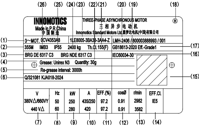
1LE8 铸铁系列电机铭牌 1LE8 Cast iron motor nameplate
